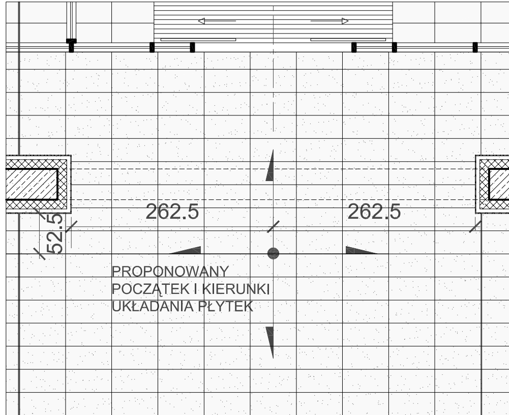
DETAL "C"
